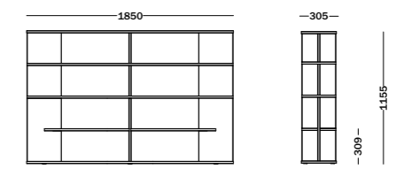
MODULE 4 - High bookshelf
