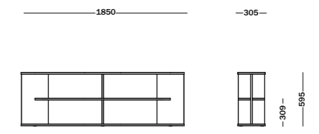
MODULE 3 - Low bookshelf
